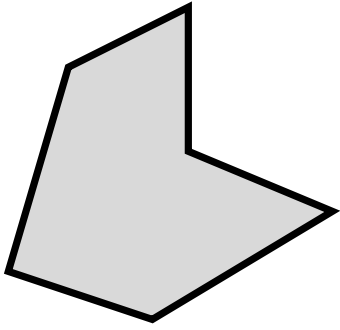
Non-convex polygon
